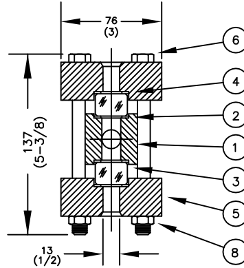
SECTION X-X SERIES T-300L
