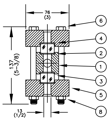
SECTION X-X SERIES T-300L
