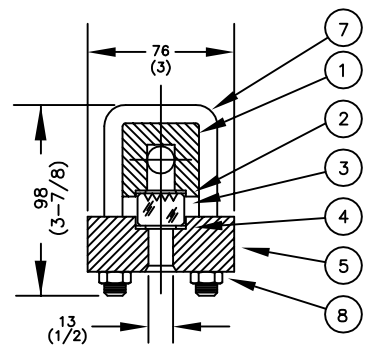
SECTION X-X SERIES R-300L
