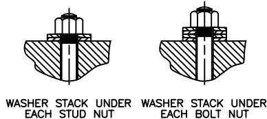
DETAIL OF WASHER STACKS
