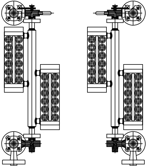
L.H. VALVE AND GAGE ASSEMBLY
