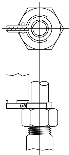
MOUNTING CLAMP FOR USE ON TUBULAR GLASS
