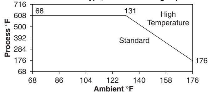
Pressure Tube Type, Non-Condensing Liquids
