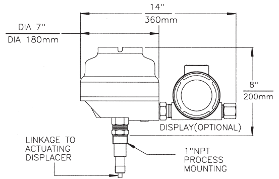
Pressure Tube Type, Non-Condensing Liquids
