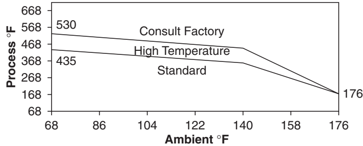
Pressure Tube Type, Condensing Liquids
