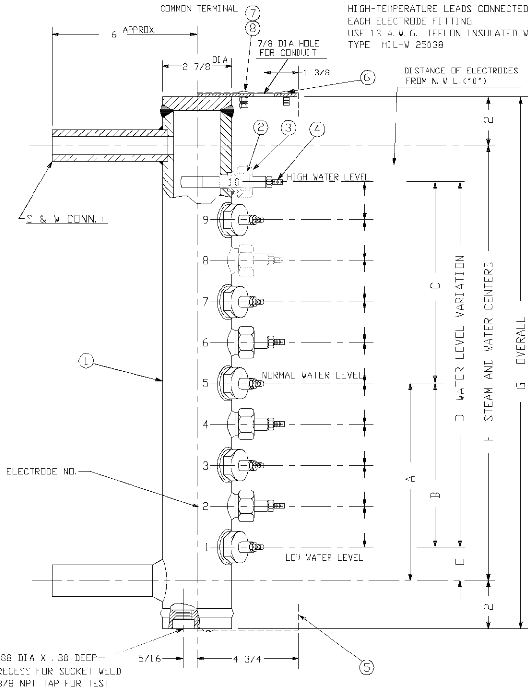
TYPICAL ARRANGEMENT
